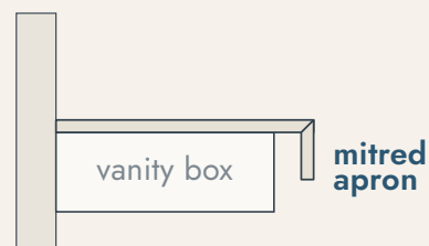
Mitred apron (section)
